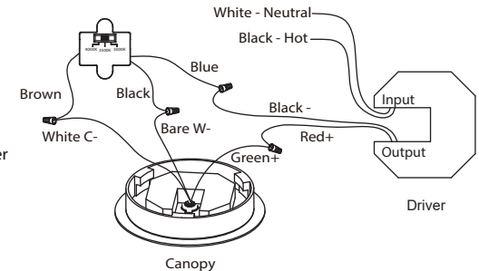
Fig. 3 Wire Diagram
